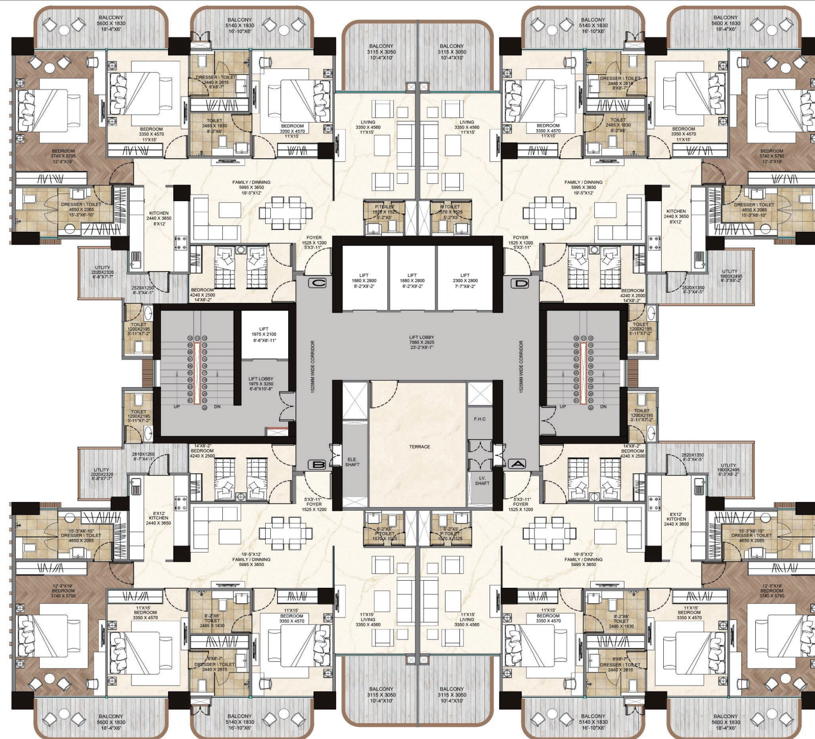
1 st FLOOR PLAN ROAD SIDE
